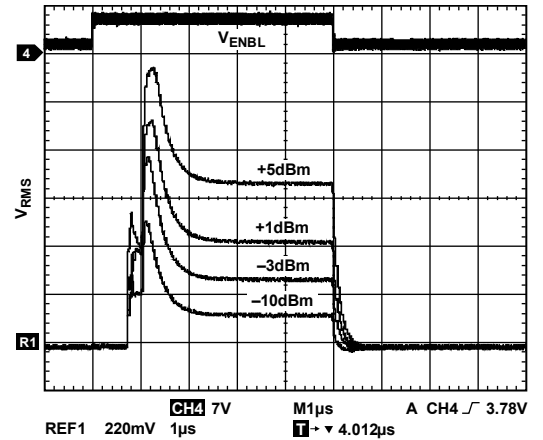
Figure 44. V_{RMS} Output Response to Enable Gating at Various RF Input Levels, 900 MHz Frequency, C_{FLT4} = \text{Open}
