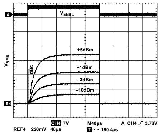
Figure 45. V_{RMS} Output Response to Enable Gating at Various RF Input Levels, 900 MHz Frequency, C_{FLT4} = 100 \text{ nF}
